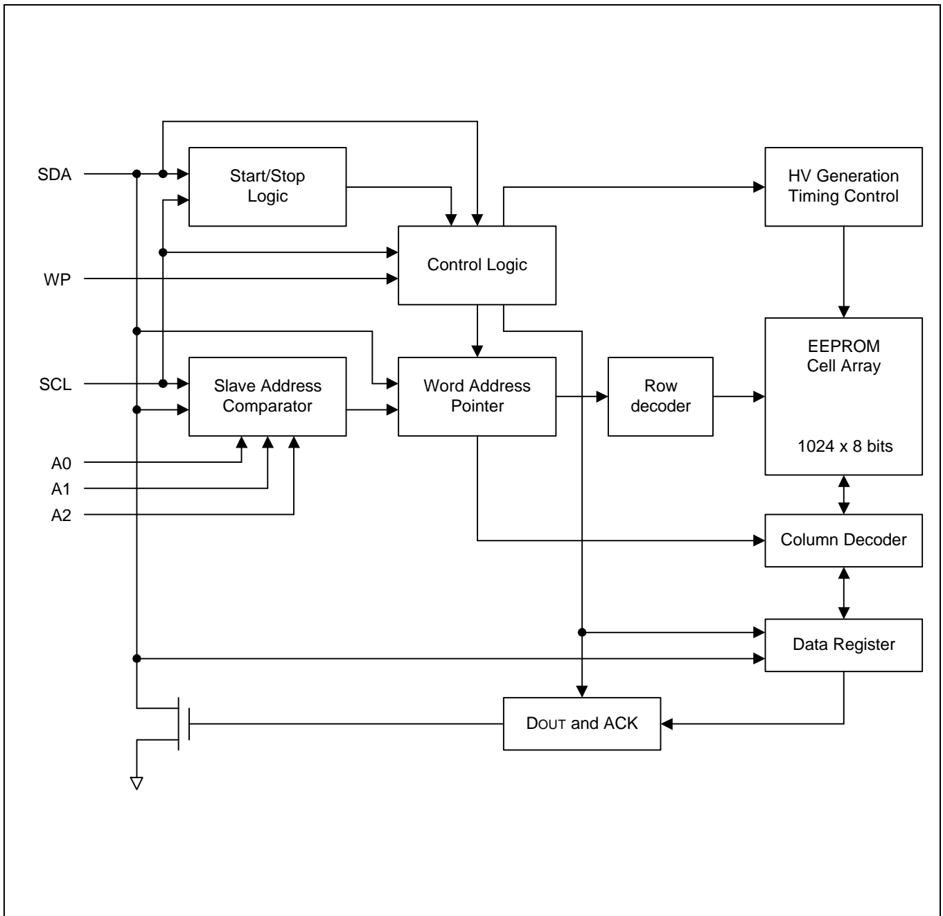
Figure 3-1. 24A08 Block Diagram
